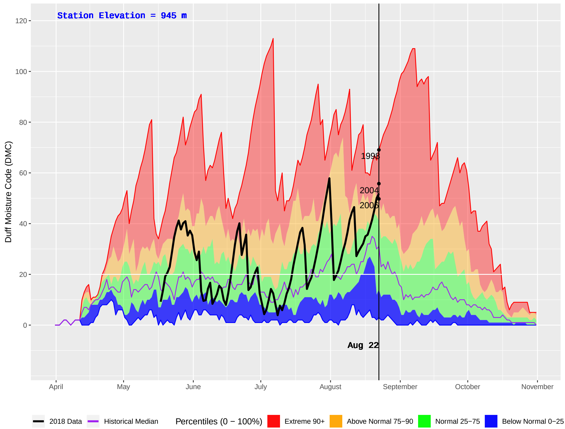
BOWRON HAGGEN (193) : Historical (1986–2016) and Current (2018) Daily Duff Moisture Code (DMC)
