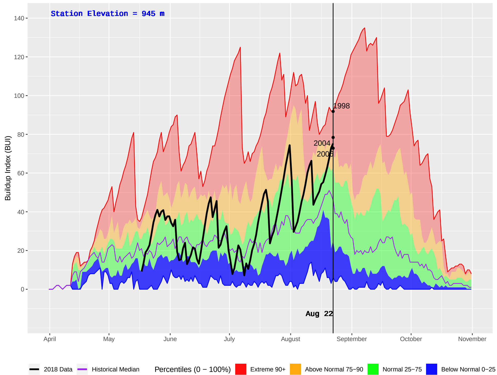
BOWRON HAGGEN (193) : Historical (1986–2016) and Current (2018) Daily Buildup Index (BUI)
